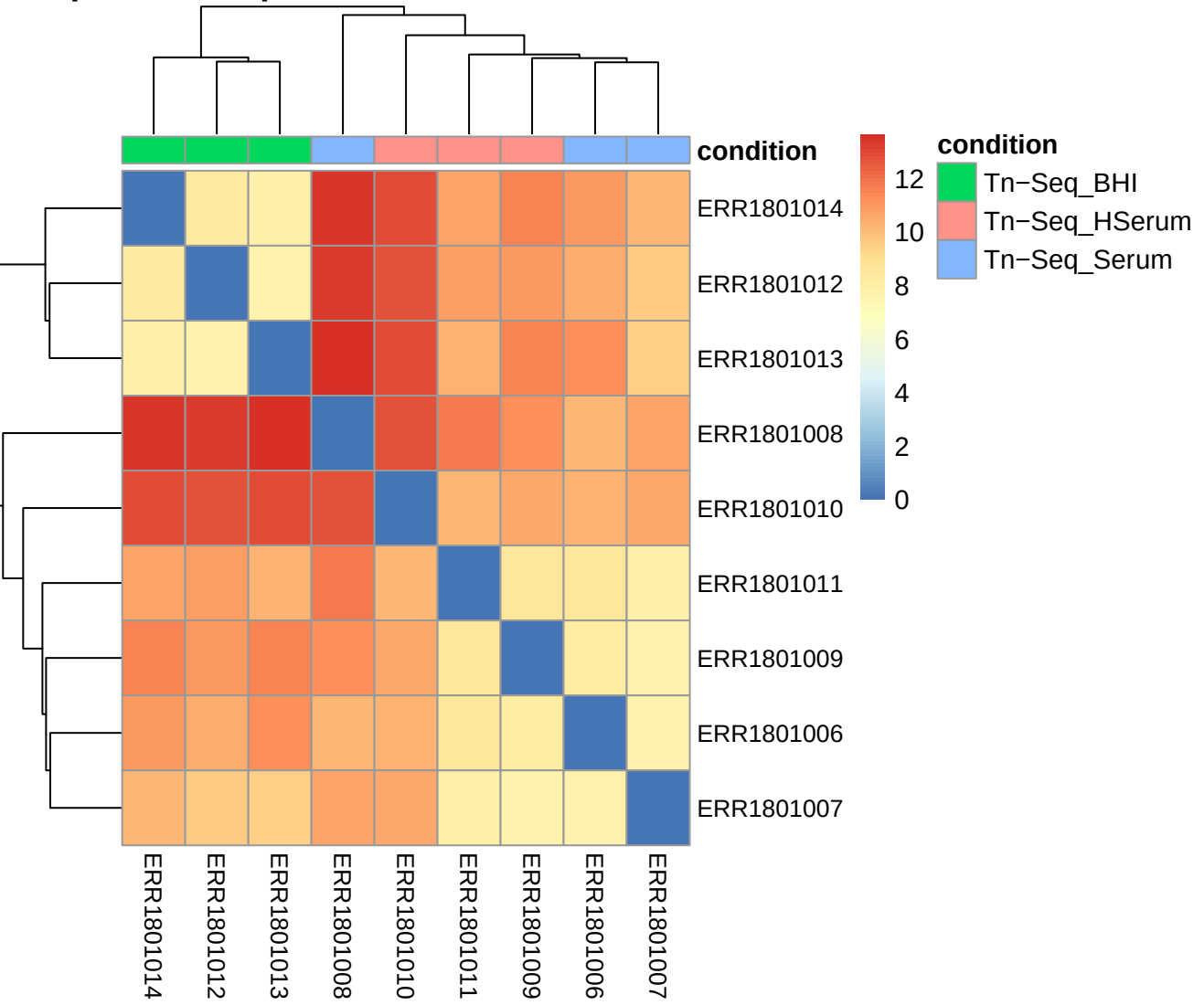
Sample-to-sample distance based on VST counts
